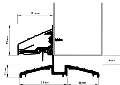
TK threshold with WA weatherboard
