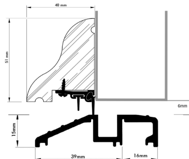
TJ Threshold with WC weatherboard
