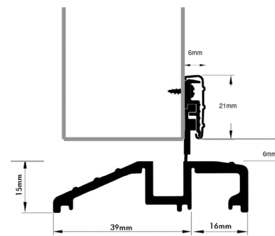
TJ threshold with CA contact strip
