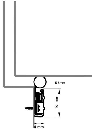
SC Holder with 093 Insert
