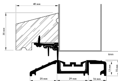
TA Threshold with WB weatherboard
