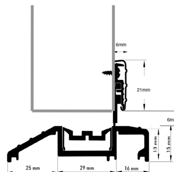
TA threshold with CA contact strip
