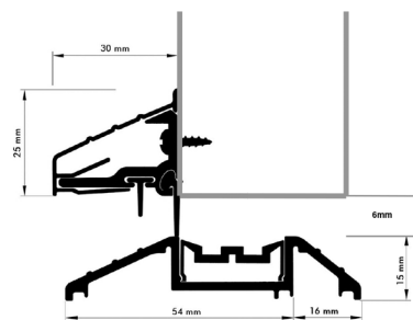
TB threshold with WA weatherboard
