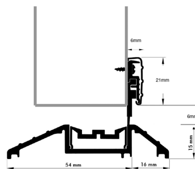
TB threshold with CA contact strip
