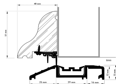
TA Threshold with WC weatherboard
