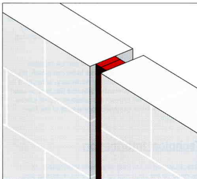
Firefoam vertical joint.
